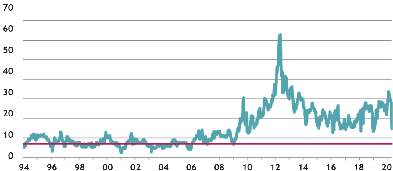
Figure 10.2 - U.S. Based Petrochemical Competitiveness: Ratio of the Price of Oil (Brent) to Natural Gas (Henry Hub)
